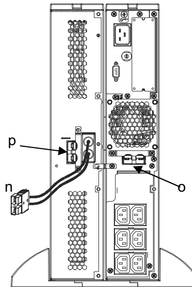
Battery Pack UPS Rear View
